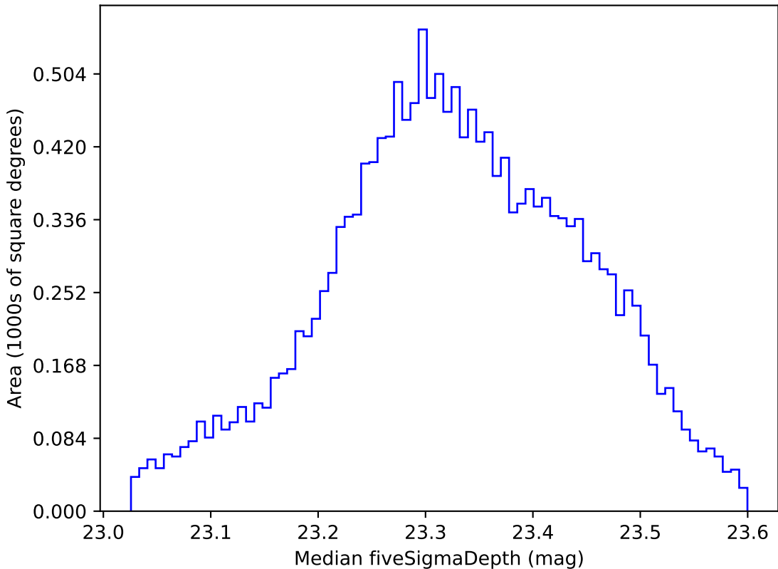
too_ignore_5_1v3.4_10yrs WFD all bands: Median fiveSigmaDepth
