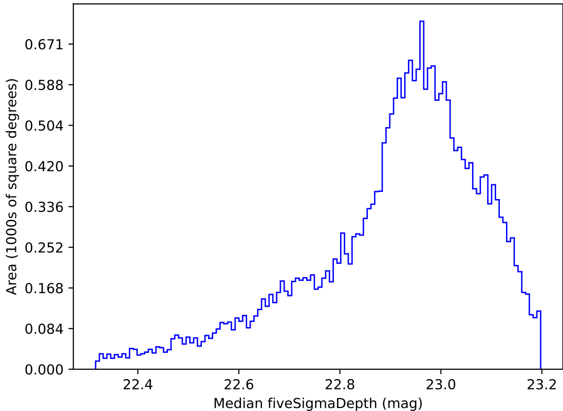
too_ignore_5_1v3.4_10yrs All sky z band: Median fiveSigmaDepth
