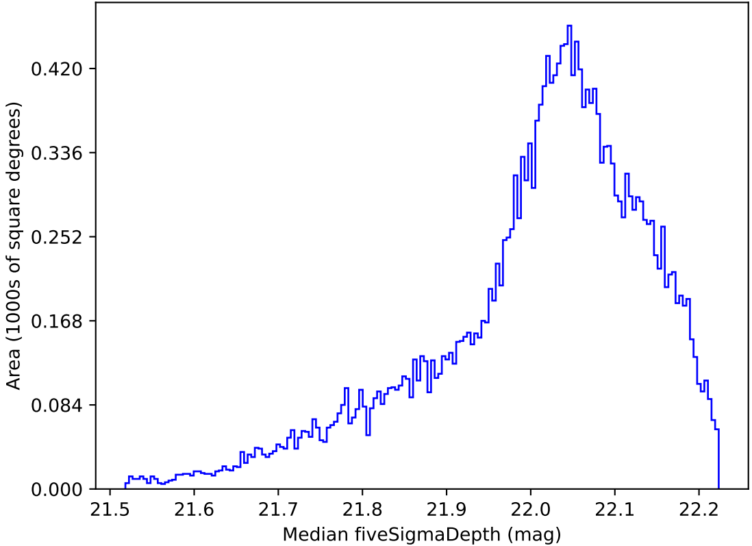
too_ignore_5_1v3.4_10yrs All sky y band: Median fiveSigmaDepth
