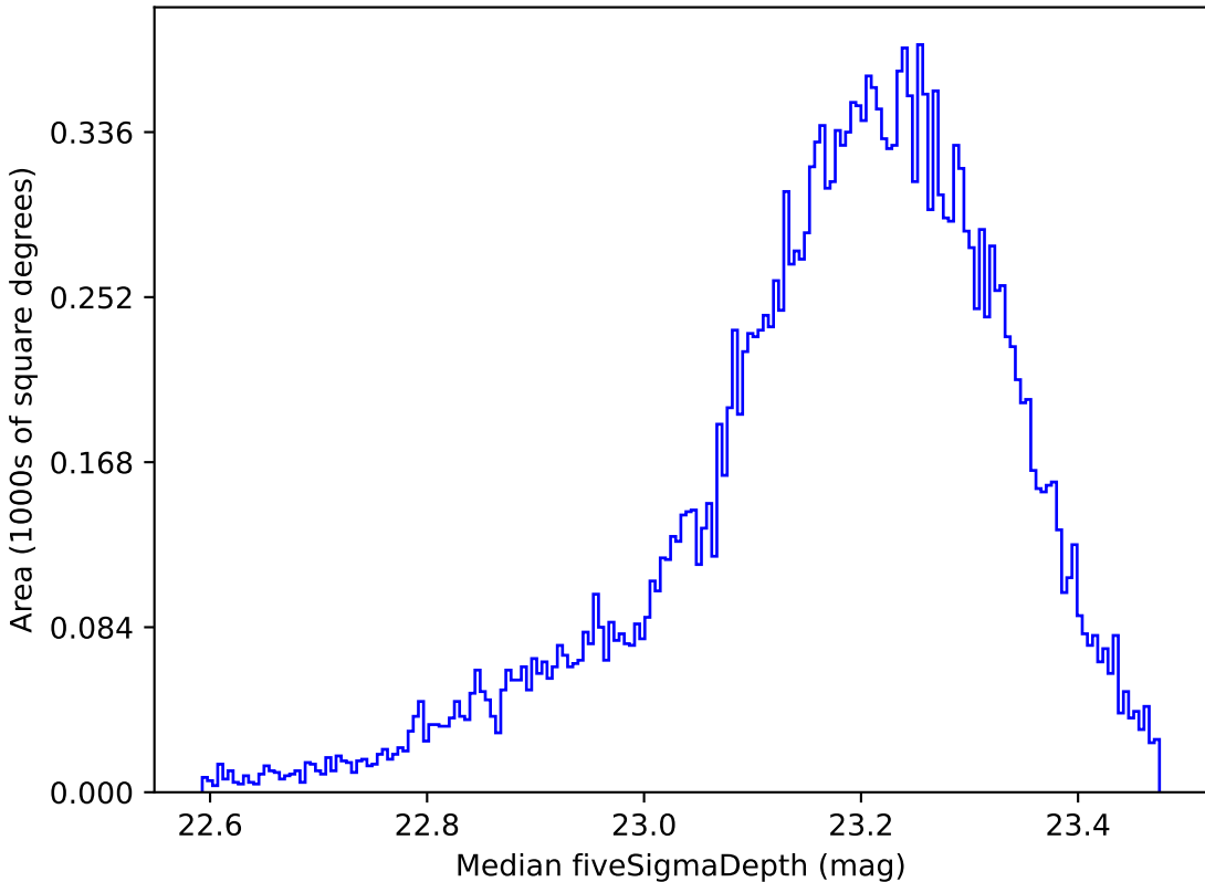
too_ignore_5_1v3.4_10yrs All sky u band: Median fiveSigmaDepth
