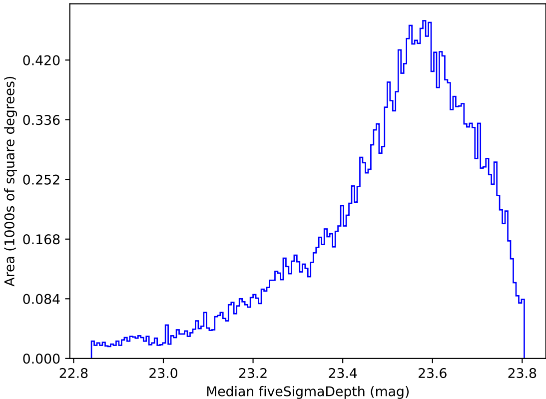
too_ignore_5_1v3.4_10yrs All sky i band: Median fiveSigmaDepth
