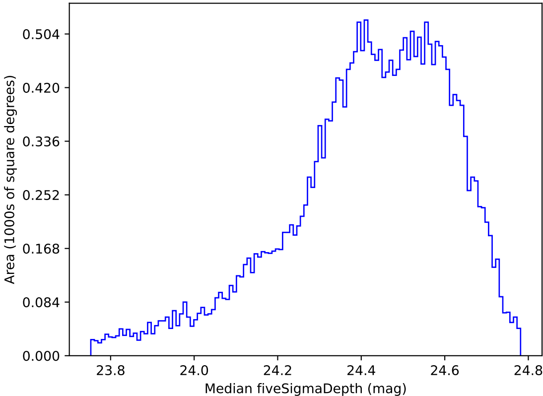
too_ignore_5_1v3.4_10yrs All sky g band: Median fiveSigmaDepth
