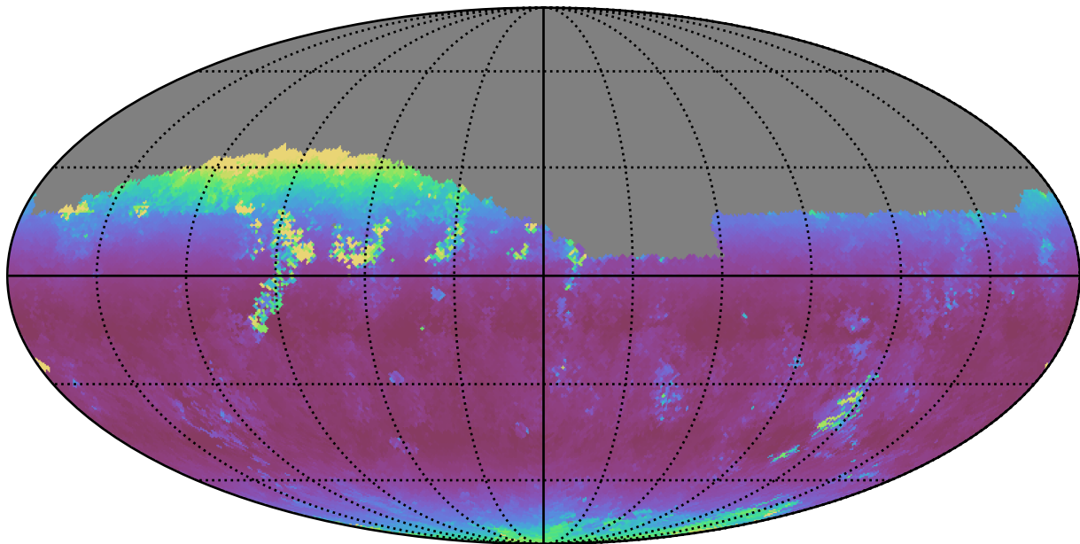
too_ignore_5_1v3.4_10yrs Yr 1 z band: Median airmass
