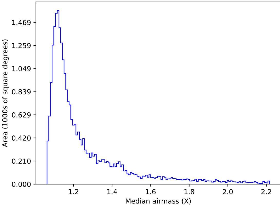
too_ignore_5_1v3.4_10yrs Yr 1 z band: Median airmass
