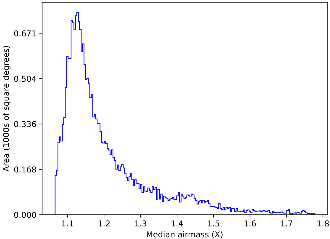
too_ignore_5_1v3.4_10yrs Yr 1 y band: Median airmass
