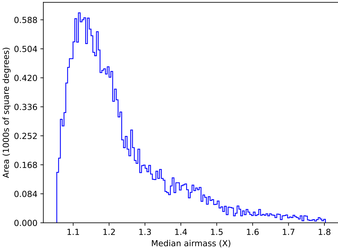
too_ignore_5_1v3.4_10yrs Yr 1 u band: Median airmass
