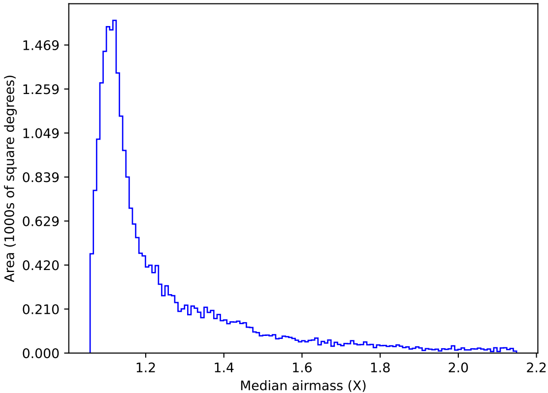
too_ignore_5_1v3.4_10yrs Yr 1 r band: Median airmass
