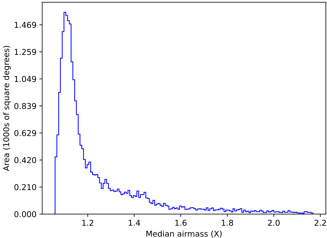
too_ignore_5_1v3.4_10yrs Yr 1 i band: Median airmass
