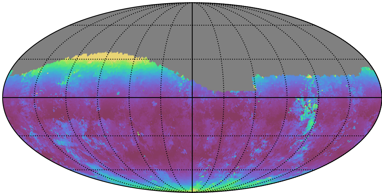
too_ignore_5_1v3.4_10yrs Yr 1 g band: Median airmass
