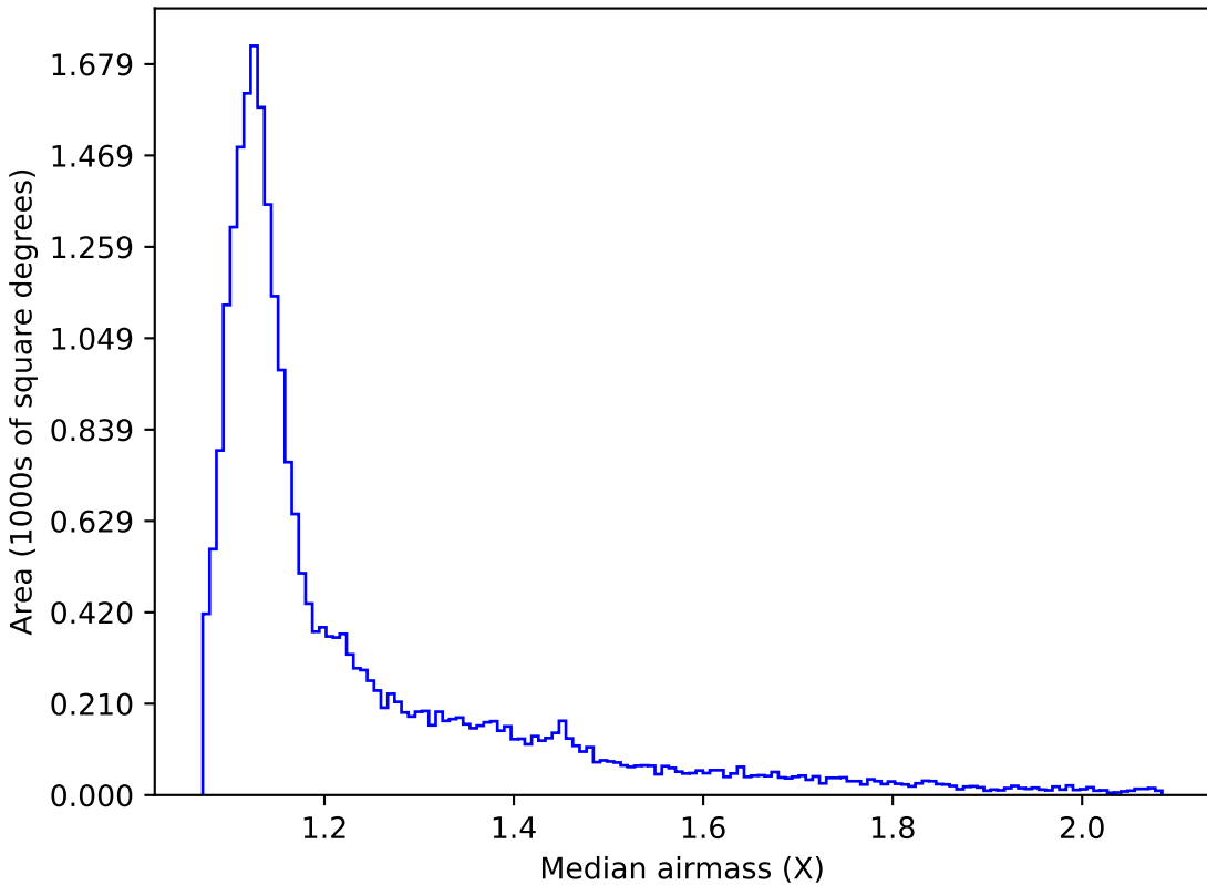
too_ignore_5_1v3.4_10yrs Yr 1 all bands: Median airmass
