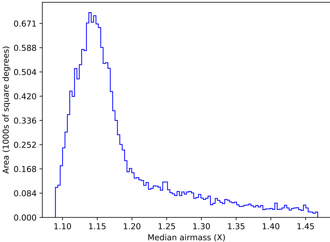
too_ignore_5_1v3.4_10yrs WFD z band: Median airmass
