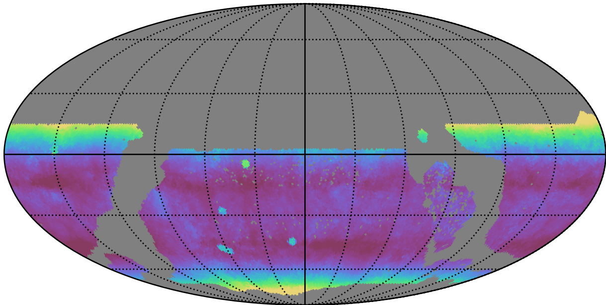
too_ignore_5_1v3.4_10yrs WFD y band: Median airmass
