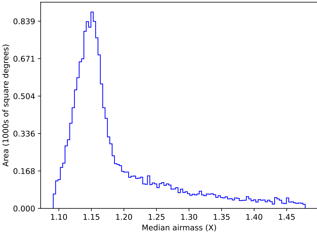
too_ignore_5_1v3.4_10yrs WFD y band: Median airmass
