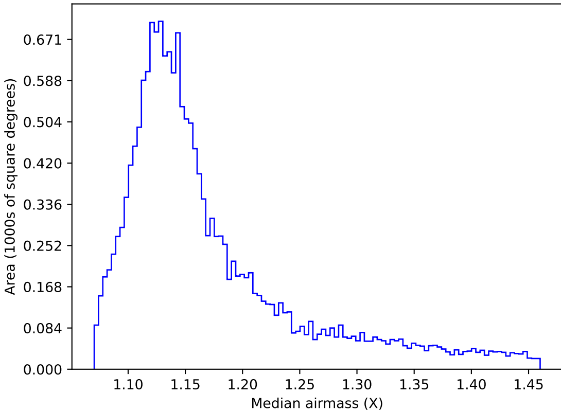
too_ignore_5_1v3.4_10yrs WFD u band: Median airmass
