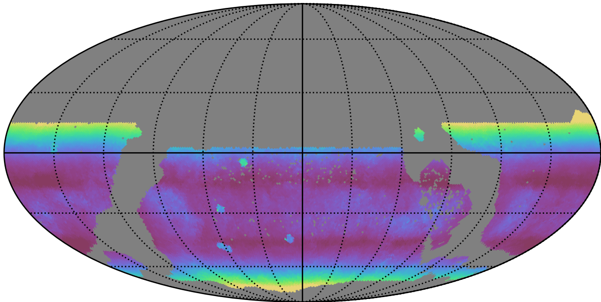
too_ignore_5_1v3.4_10yrs WFD r band: Median airmass
