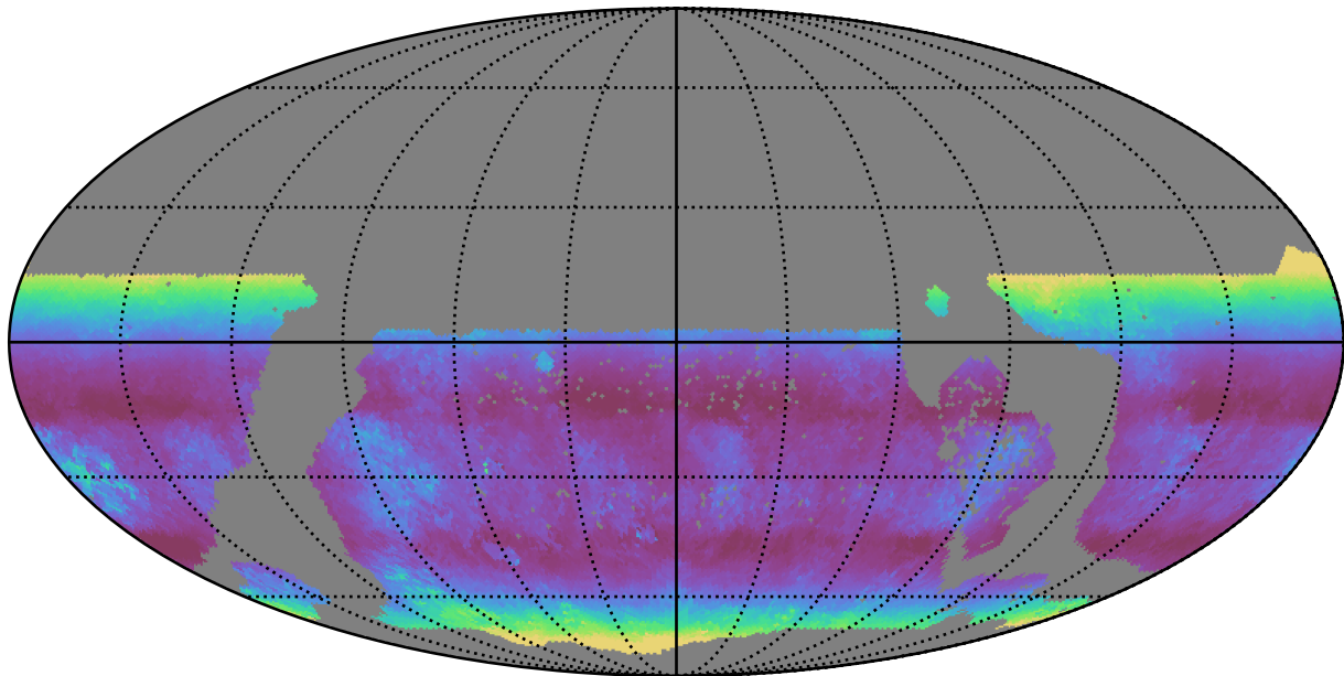
too_ignore_5_1v3.4_10yrs WFD g band: Median airmass
