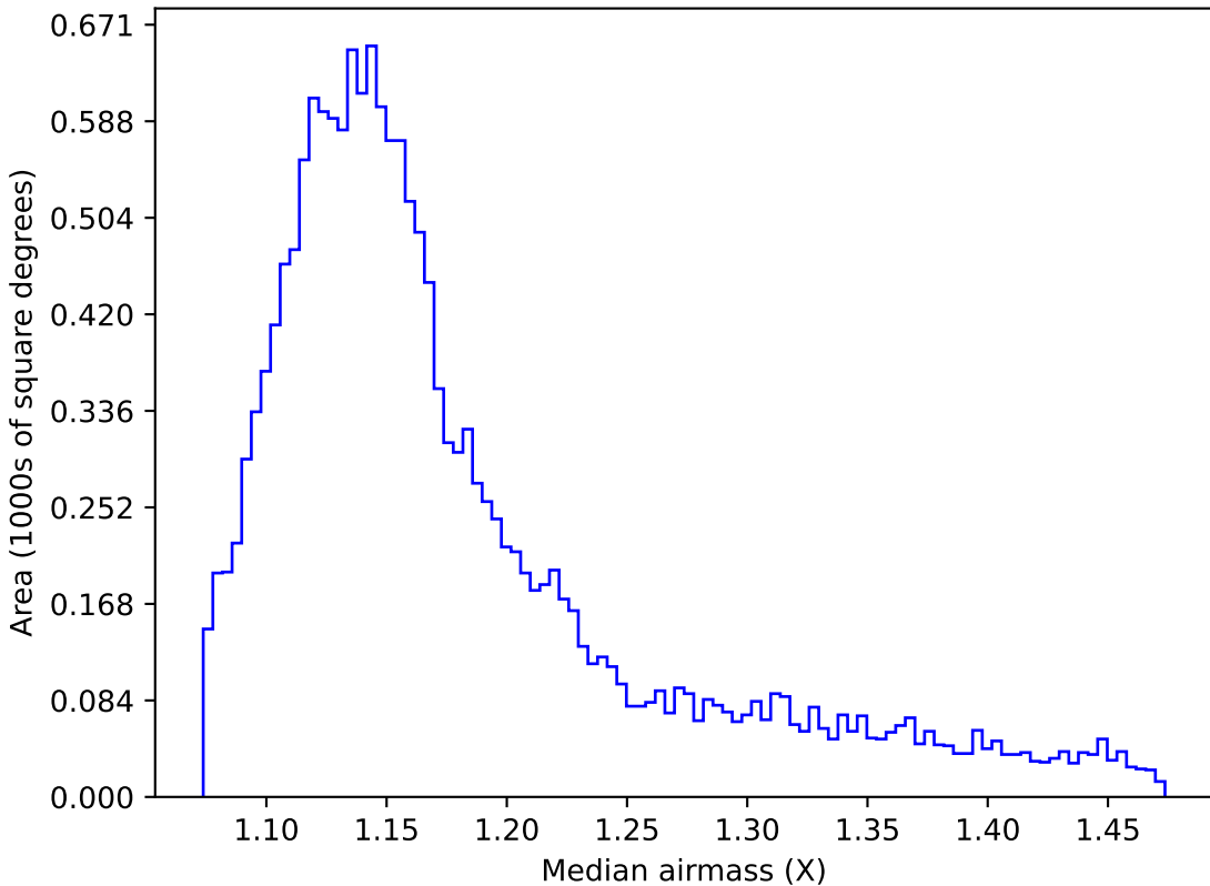
too_ignore_5_1v3.4_10yrs WFD g band: Median airmass
