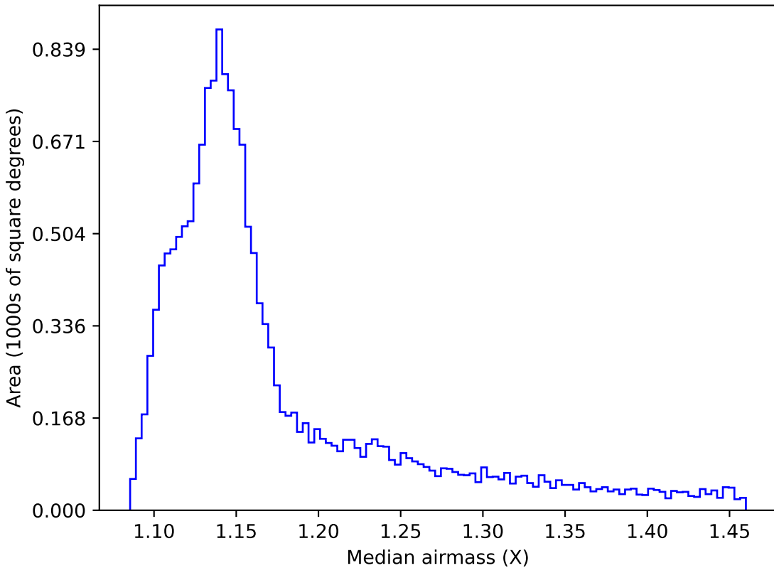
too_ignore_5_1v3.4_10yrs WFD all bands: Median airmass
