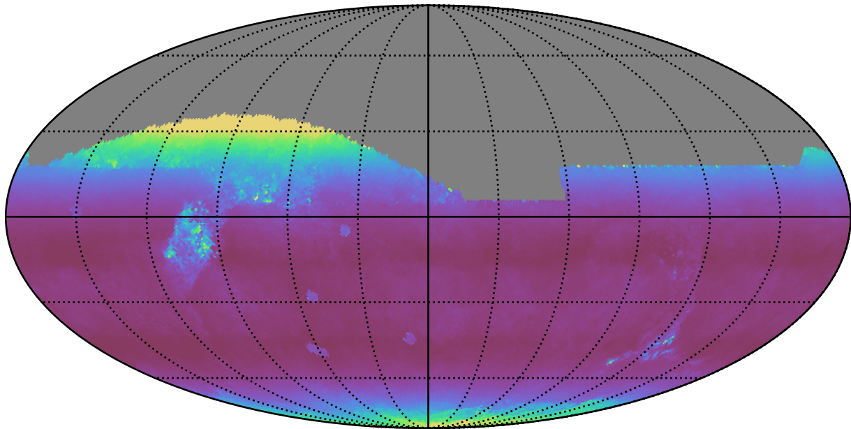
too_ignore_5_1v3.4_10yrs All sky z band: Median airmass
