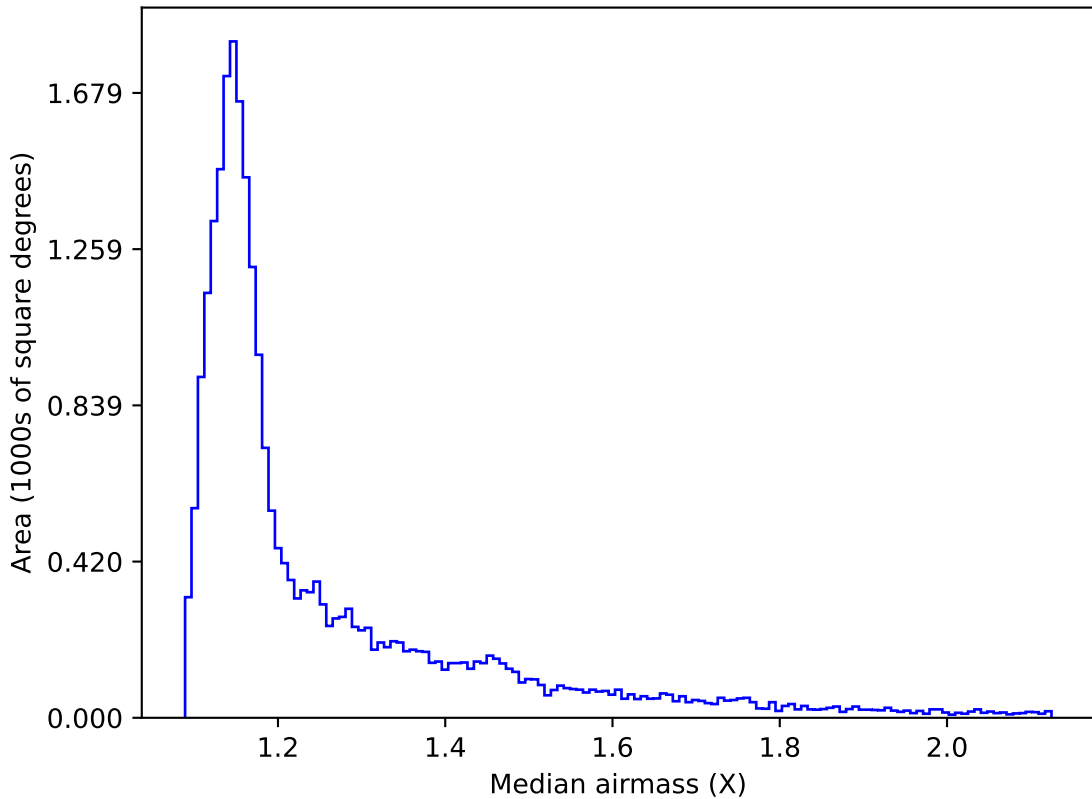
too_ignore_5_1v3.4_10yrs All sky z band: Median airmass
