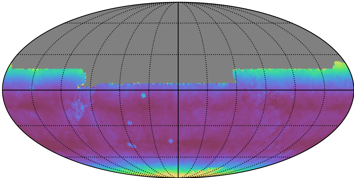
too_ignore_5_1v3.4_10yrs All sky y band: Median airmass
