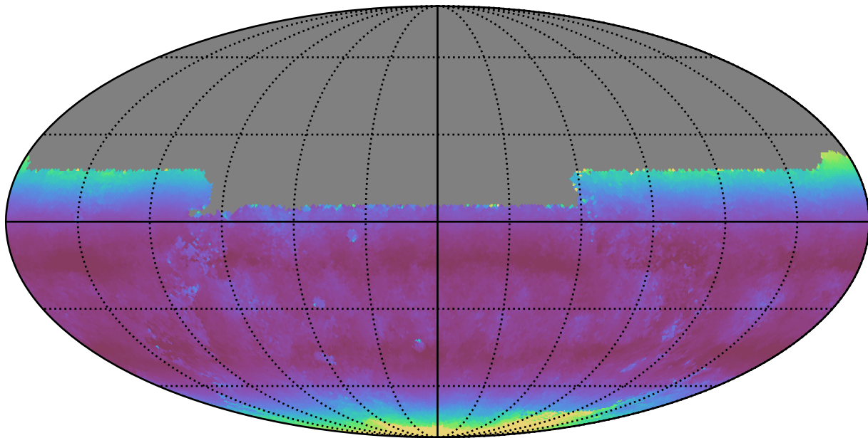
too_ignore_5_1v3.4_10yrs All sky u band: Median airmass
