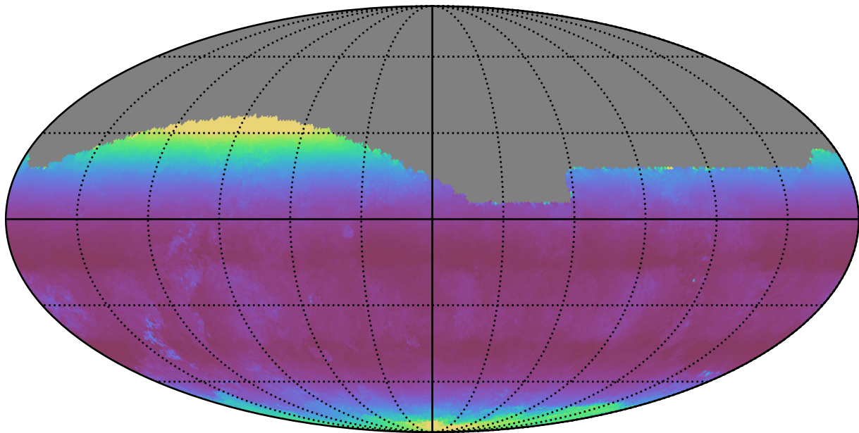
too_ignore_5_1v3.4_10yrs All sky g band: Median airmass
