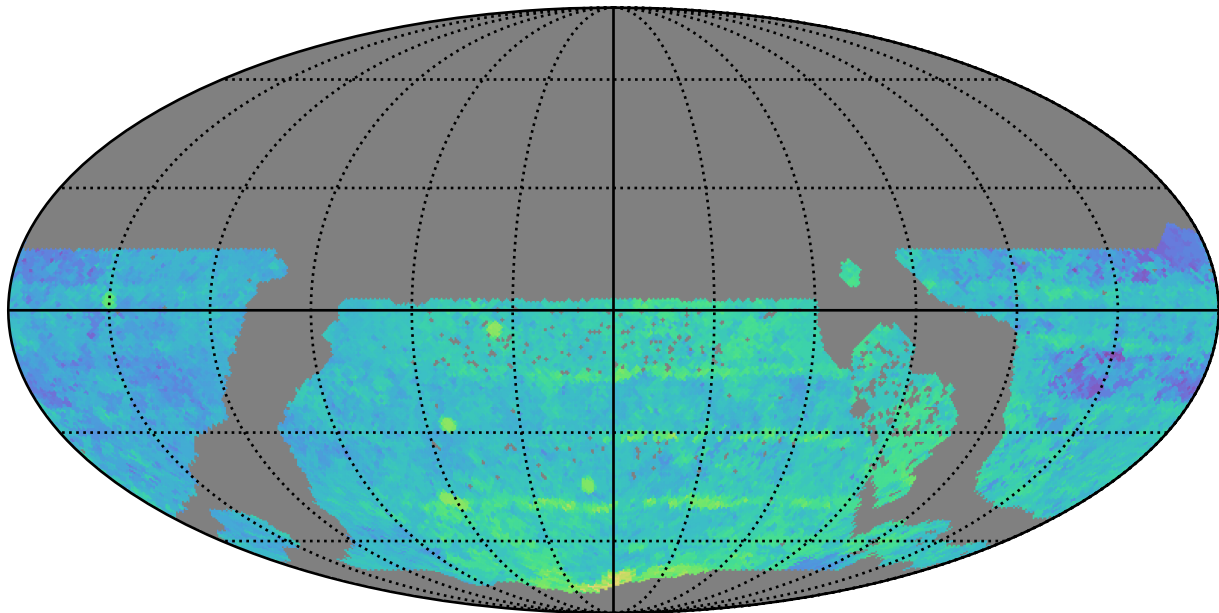
too_ignore_5_1v3.4_10yrs WFD z band: Median Season Length
