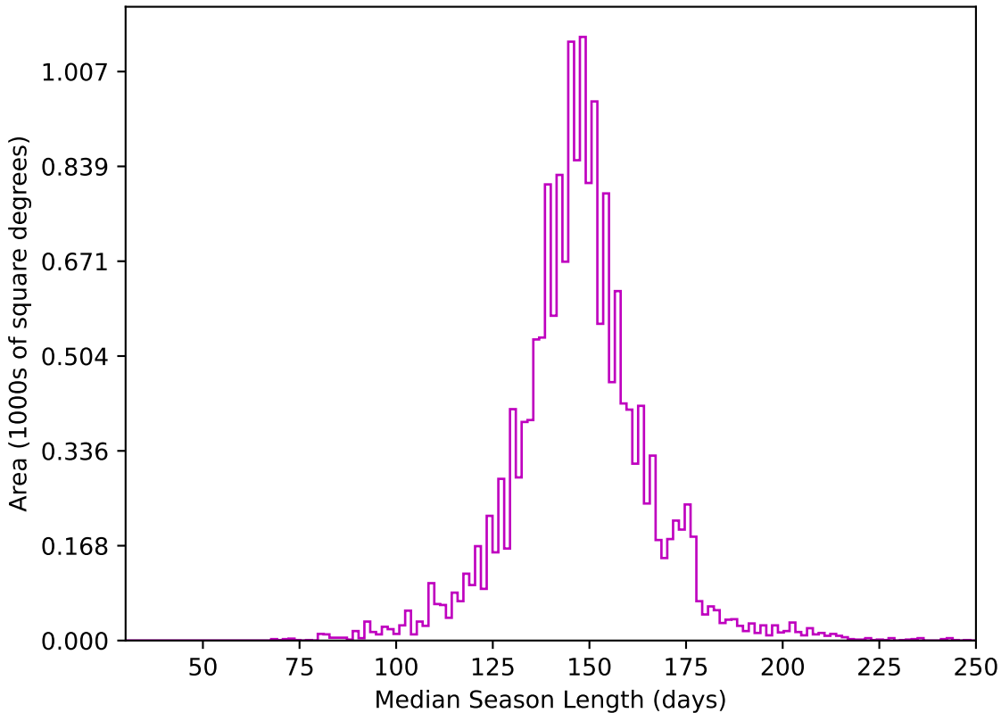
too_ignore_5_1v3.4_10yrs WFD z band: Median Season Length
