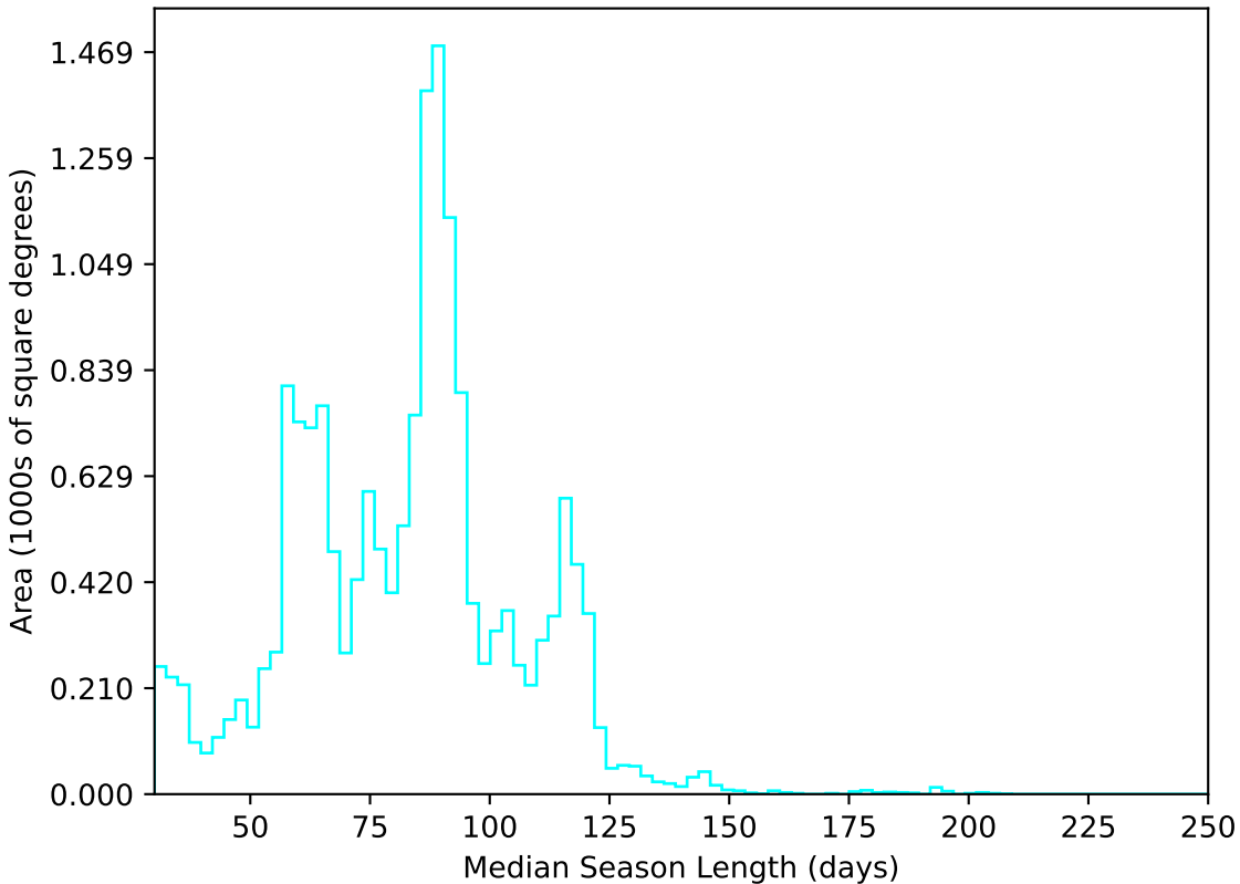
too_ignore_5_1v3.4_10yrs WFD u band: Median Season Length
