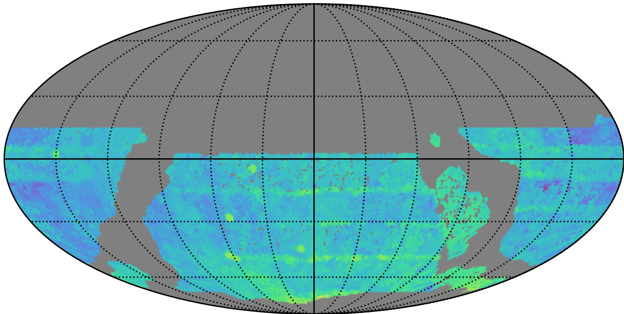
too_ignore_5_1v3.4_10yrs WFD r band: Median Season Length
