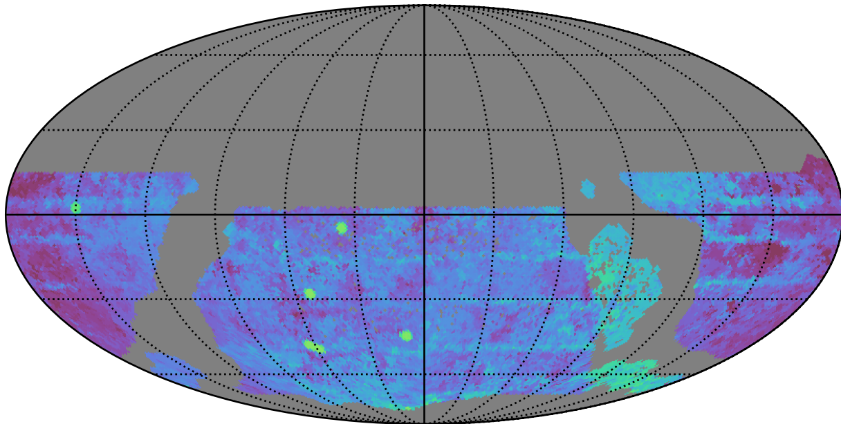
too_ignore_5_1v3.4_10yrs WFD g band: Median Season Length
