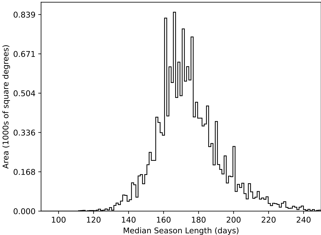
too_ignore_5_1v3.4_10yrs WFD all bands: Median Season Length
