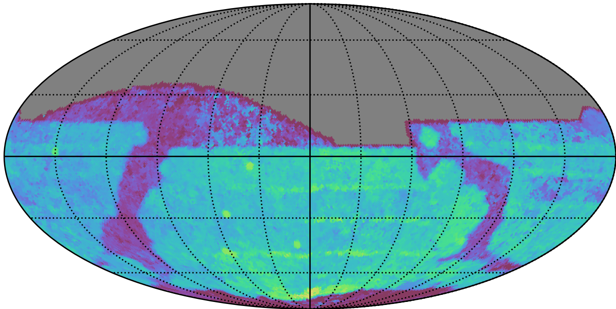
too_ignore_5_1v3.4_10yrs All sky z band: Median Season Length
