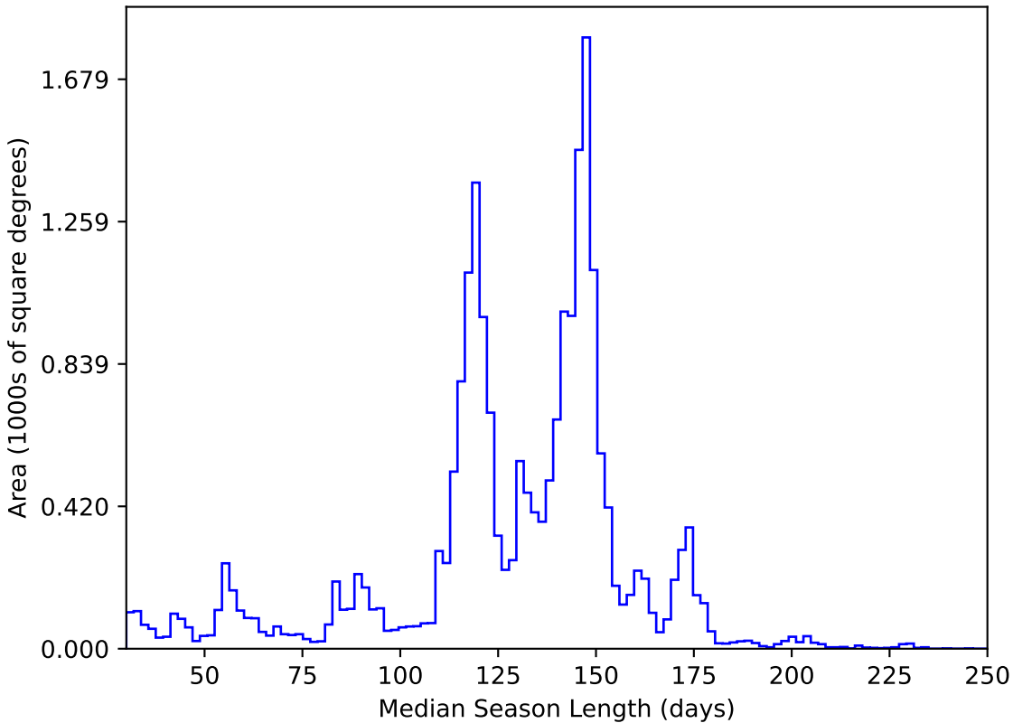
too_ignore_5_1v3.4_10yrs All sky y band: Median Season Length
