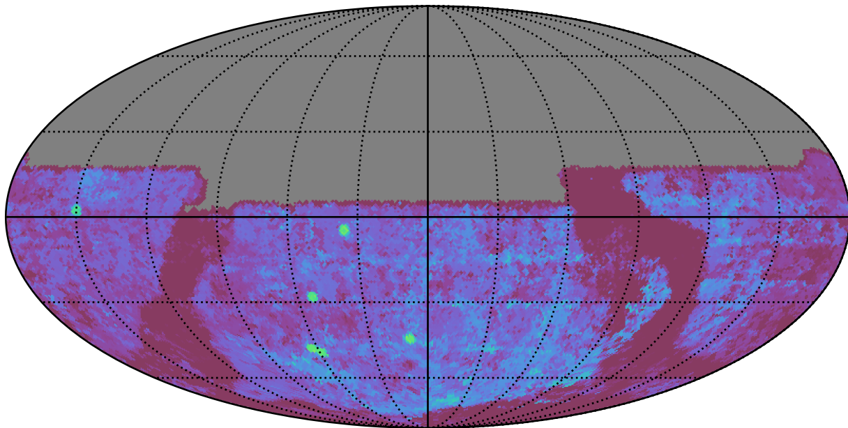
too_ignore_5_1v3.4_10yrs All sky u band: Median Season Length
