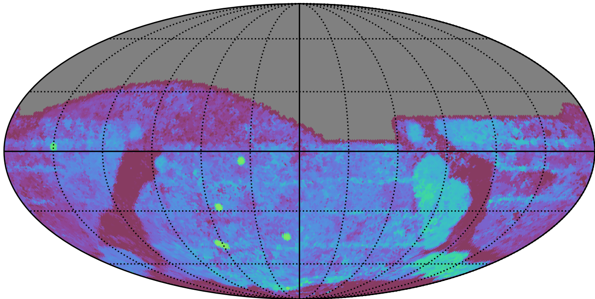
too_ignore_5_1v3.4_10yrs All sky g band: Median Season Length
