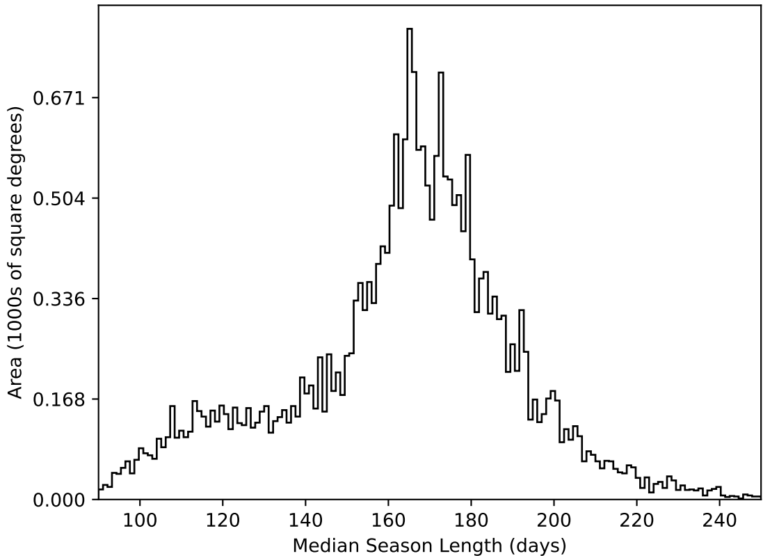
too_ignore_5_1v3.4_10yrs All sky all bands: Median Season Length
