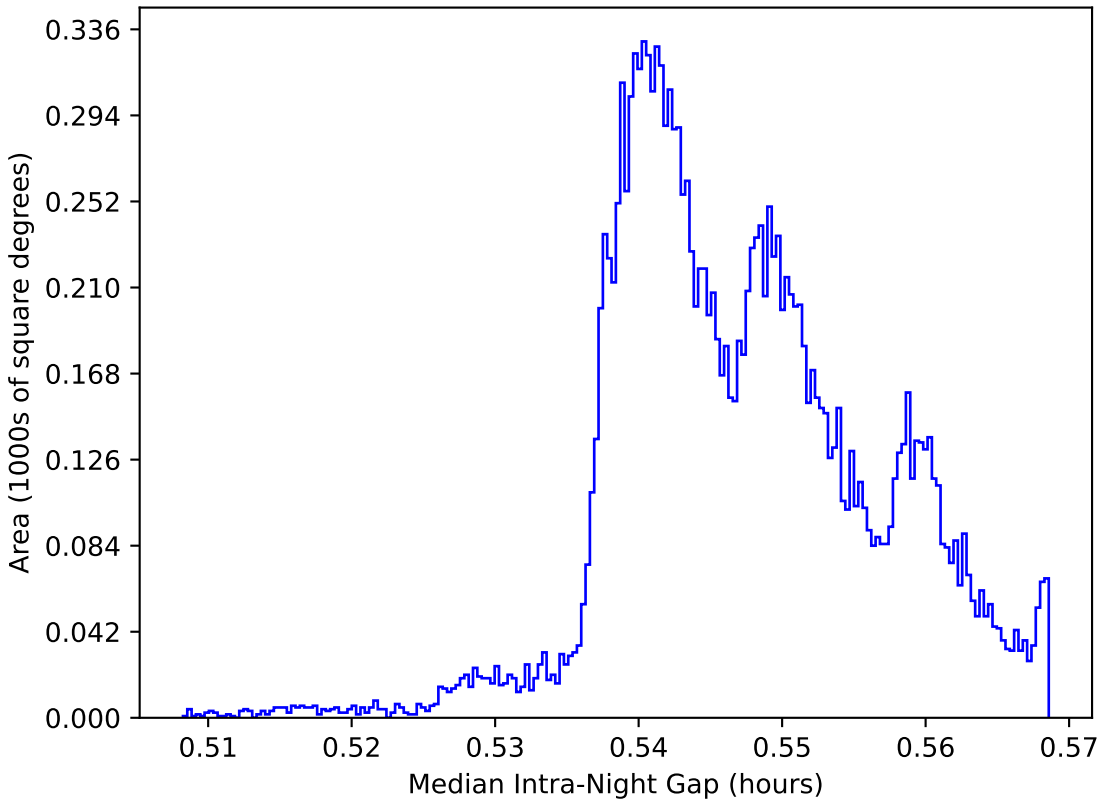
too_ignore_5_1v3.4_10yrs WFD: Median Intra-Night Gap
