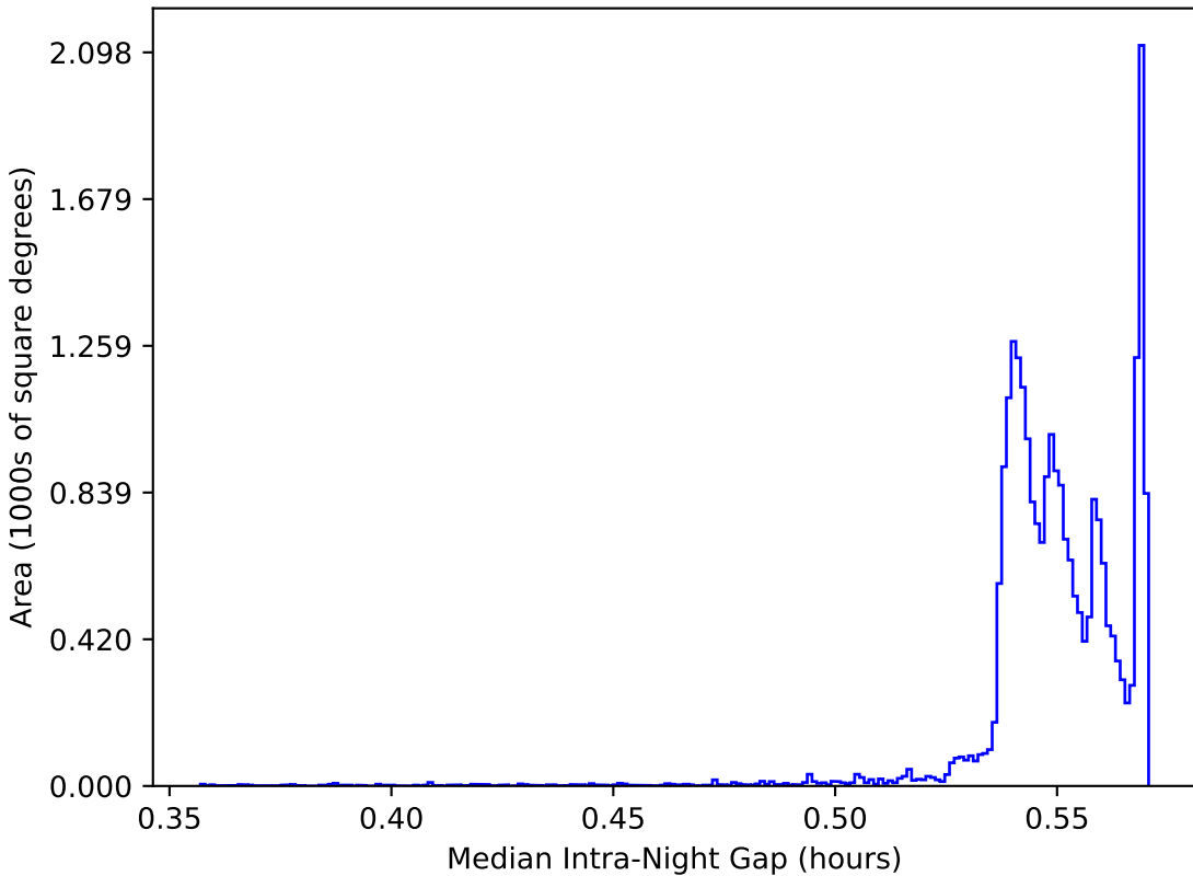
too_ignore_5_1v3.4_10yrs All sky: Median Intra-Night Gap
