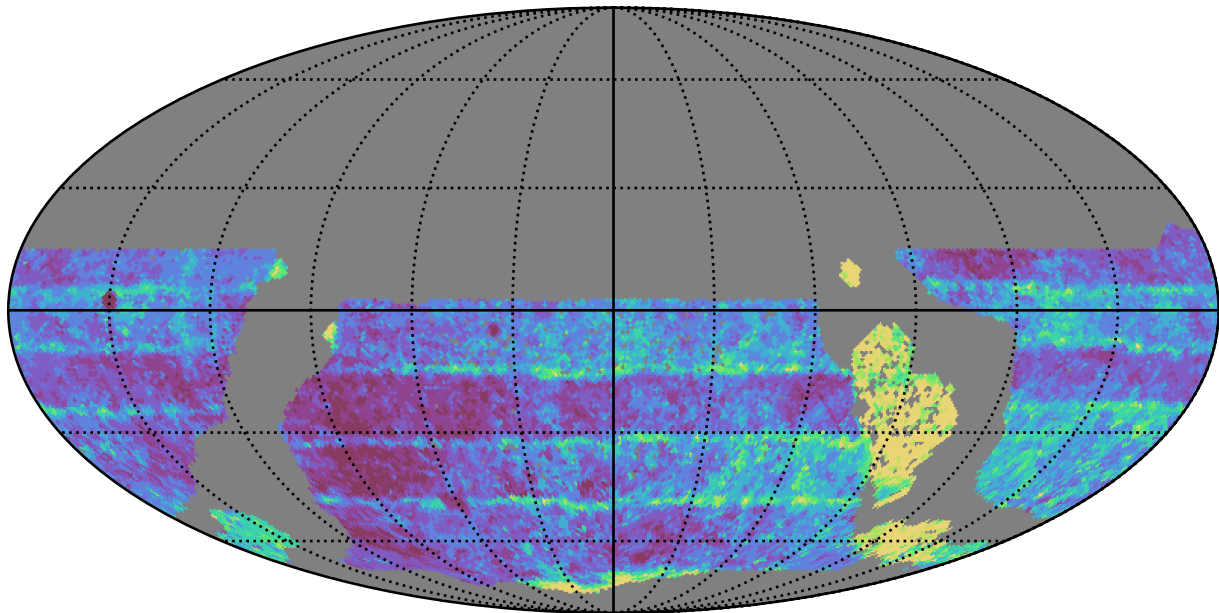
too_ignore_5_1v3.4_10yrs WFD z band: Median Inter-Night Gap
