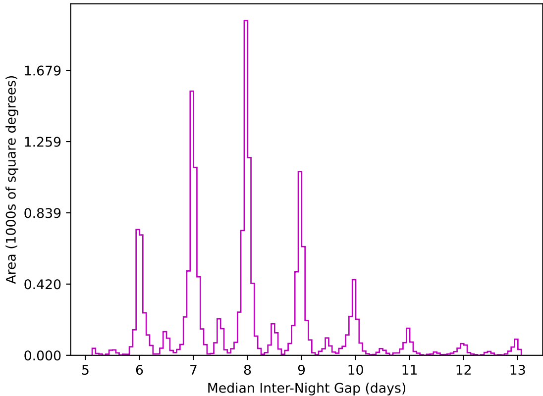
too_ignore_5_1v3.4_10yrs WFD z band: Median Inter-Night Gap
