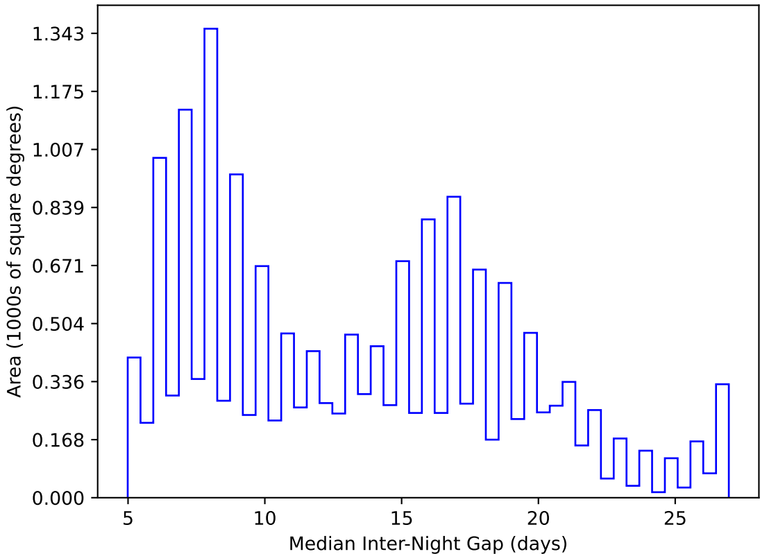
too_ignore_5_1v3.4_10yrs WFD y band: Median Inter-Night Gap
