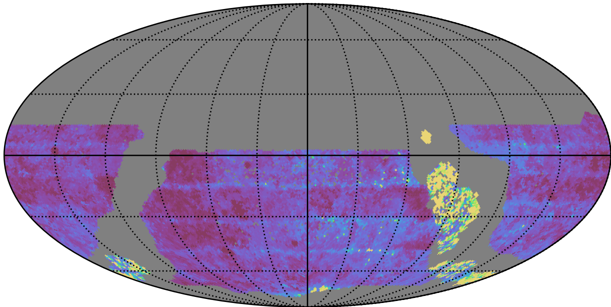
too_ignore_5_1v3.4_10yrs WFD u band: Median Inter-Night Gap
