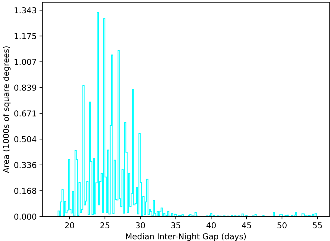
too_ignore_5_1v3.4_10yrs WFD u band: Median Inter-Night Gap
