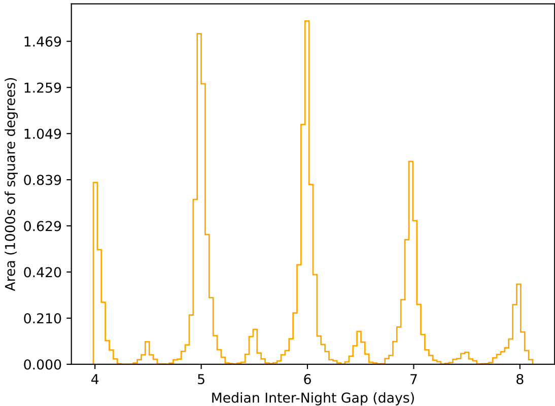
too_ignore_5_1v3.4_10yrs WFD r band: Median Inter-Night Gap
