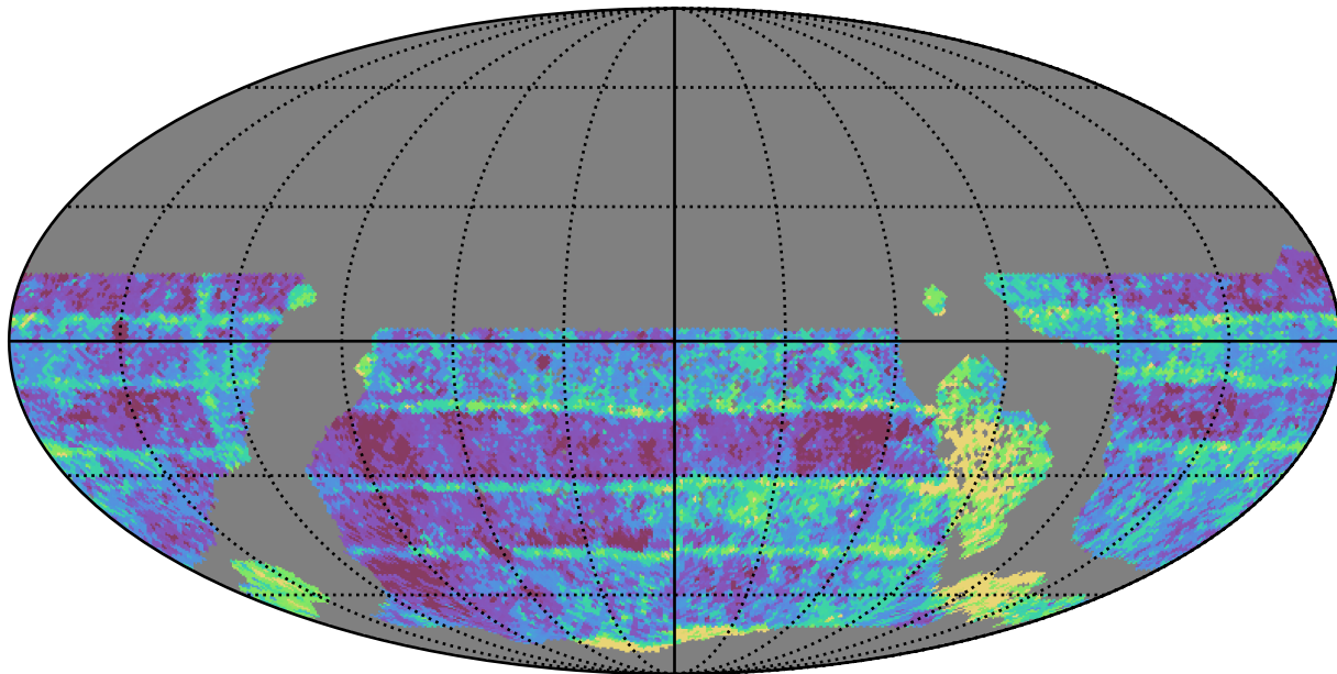
too_ignore_5_1v3.4_10yrs WFD i band: Median Inter-Night Gap
