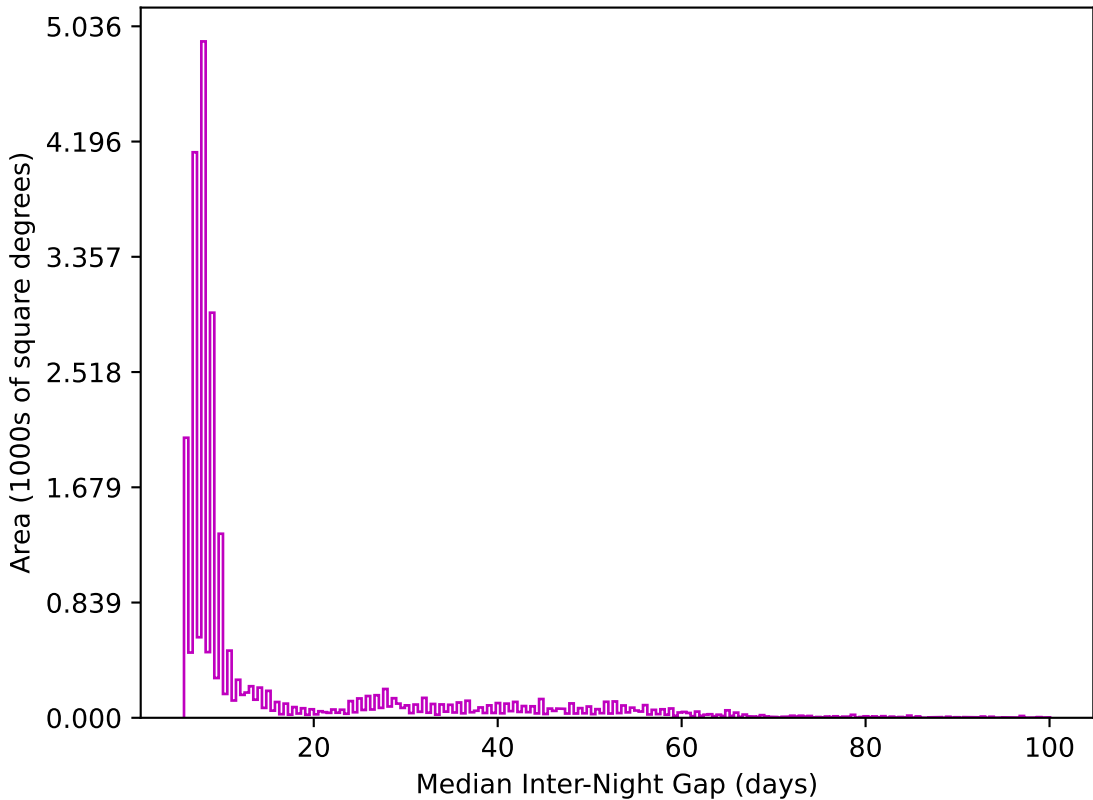
too_ignore_5_1v3.4_10yrs All sky z band: Median Inter-Night Gap
