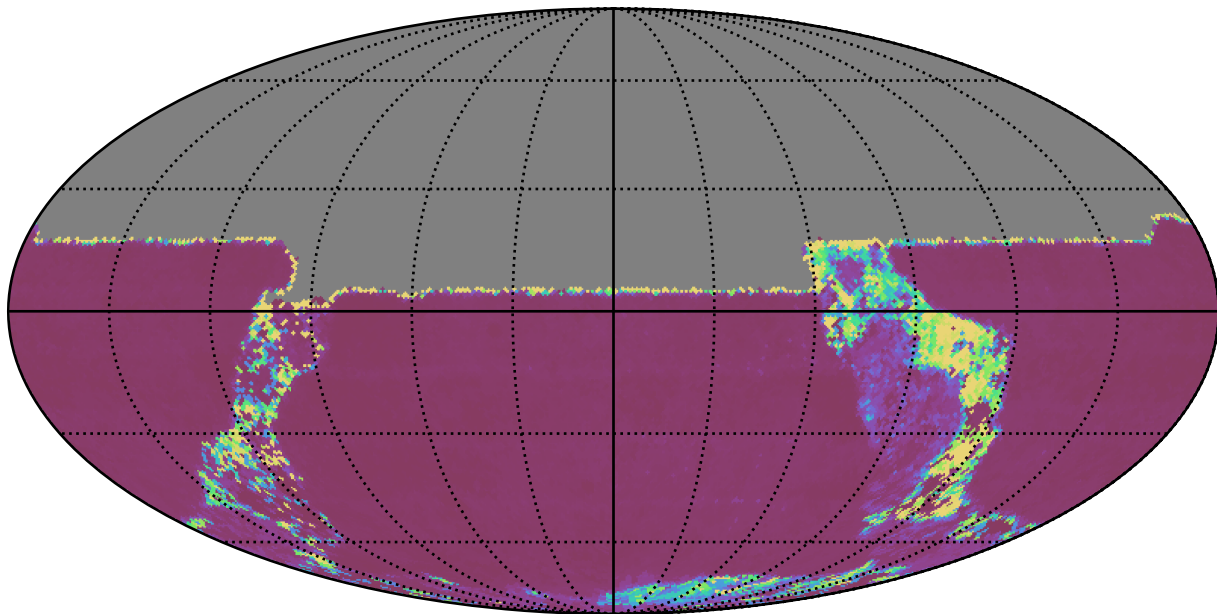
too_ignore_5_1v3.4_10yrs All sky u band: Median Inter-Night Gap
