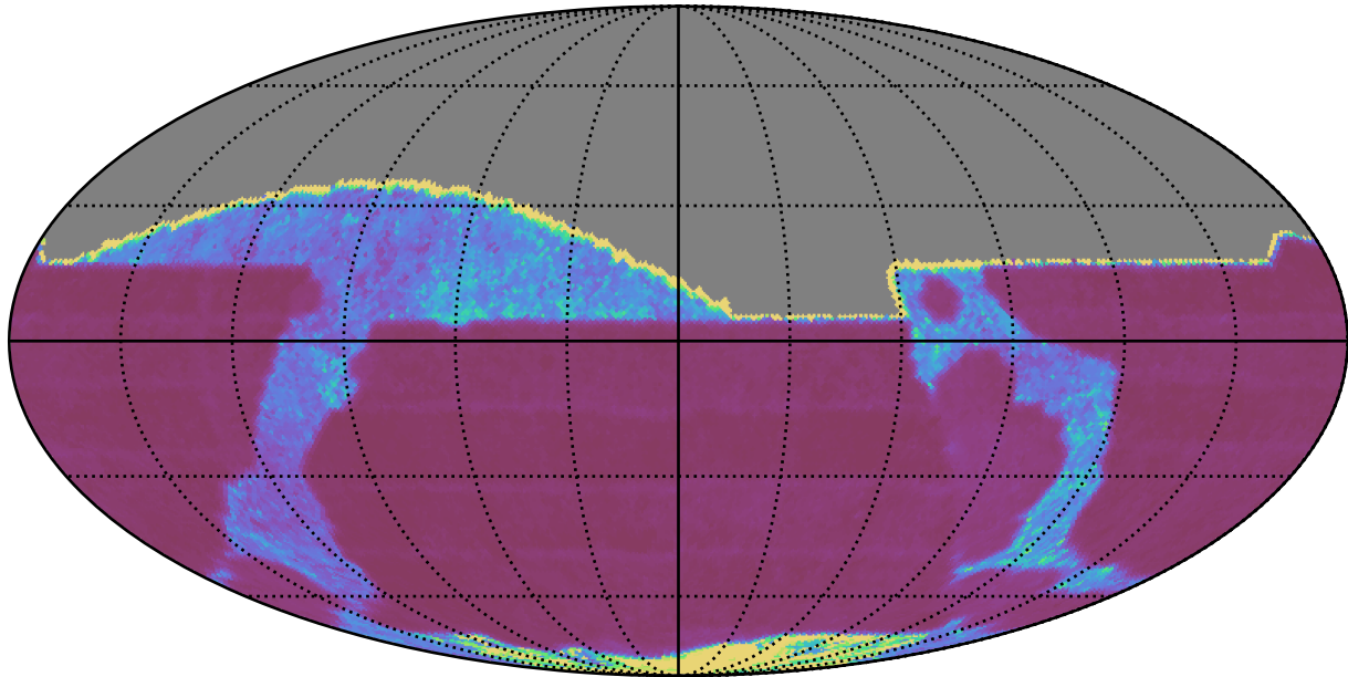
too_ignore_5_1v3.4_10yrs All sky i band: Median Inter-Night Gap
